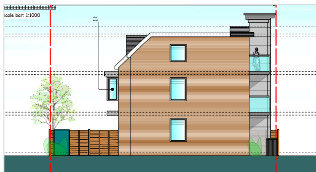
Proposed side elevation D
